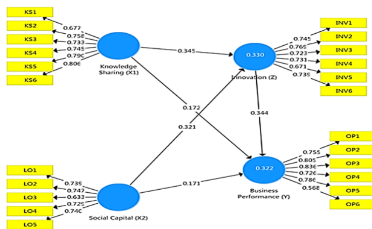
Figure 2. PLS Model
