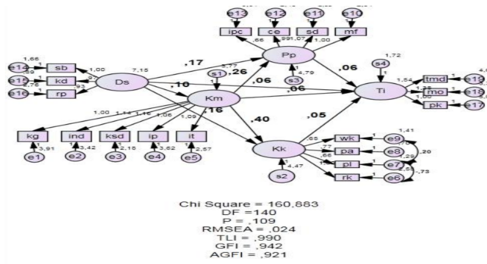
Figure2. Model two-step approach Modification to SEM
