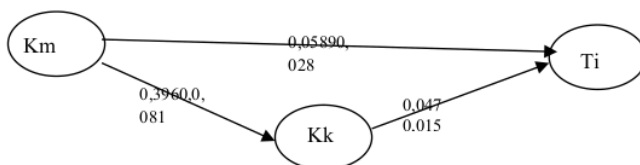
Figure 6.4. Path analysis Competency, Work Engagement, Turnover Intention
