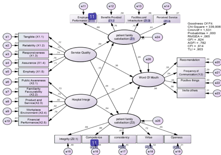
Figure 5.6. Full Structural Model
